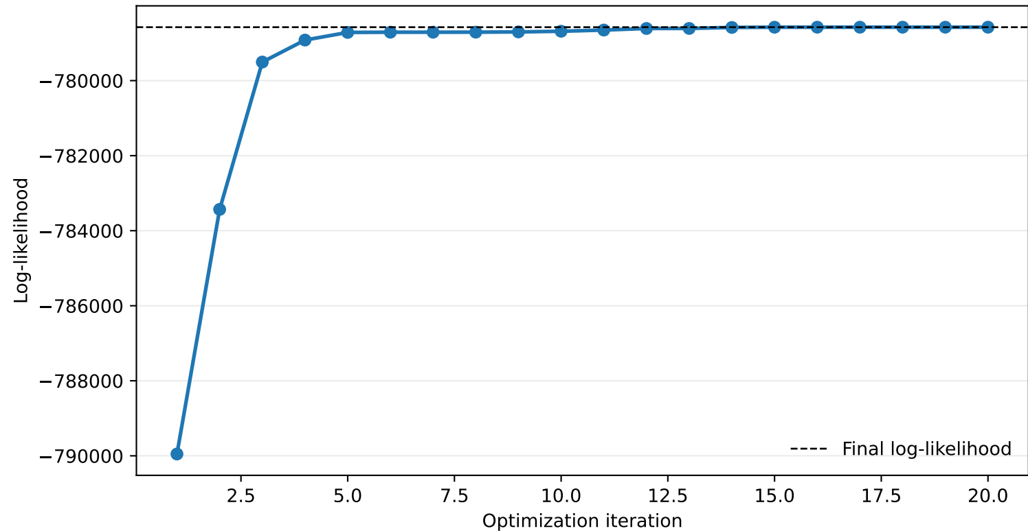
Log-likelihood over optimization iterations
